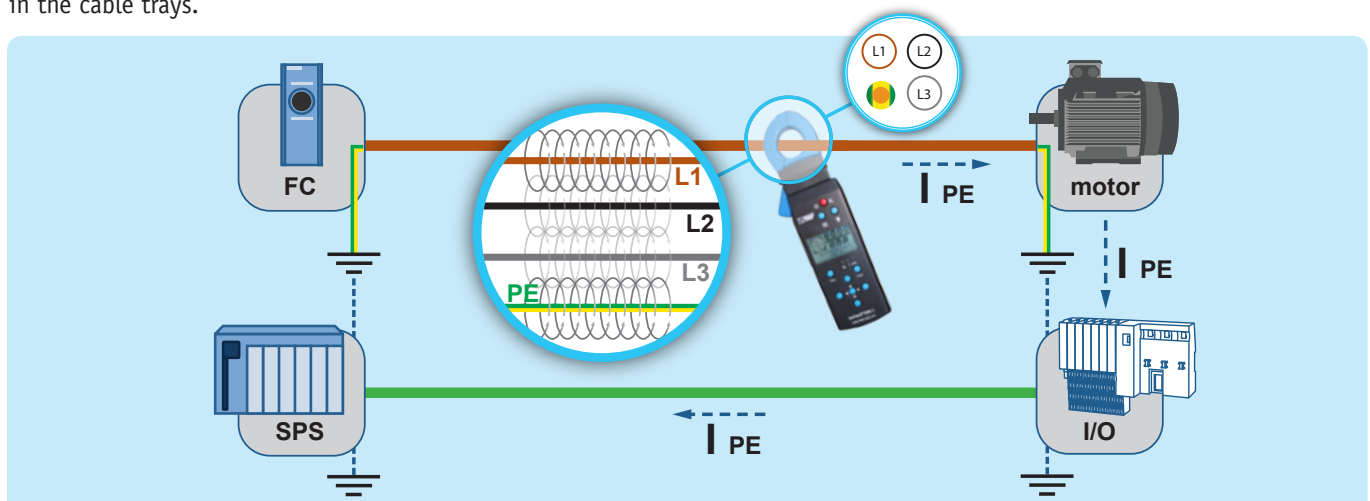
Fig. 4: Induction in the PE of motor cables
