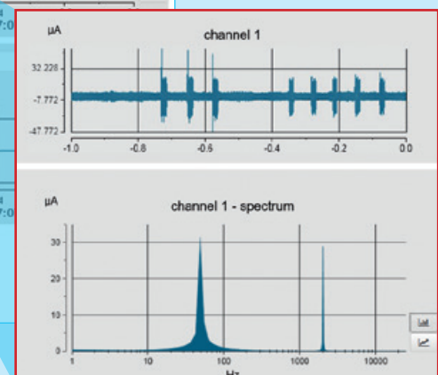
Fig. 24: Detail view of Channel 1 (amplitude, spectrum and frequency components)
